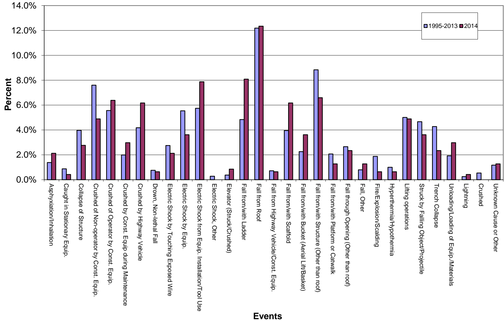
Figure B1. Comparison of Construction Fatality Events (1995-2013 with 2014)
