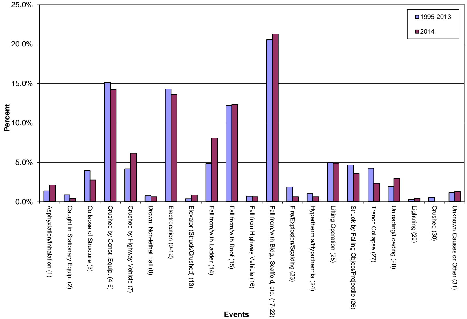
Figure B4. Comparison of Grouped Construction Fatal Events (1995-2013 and 2014)
